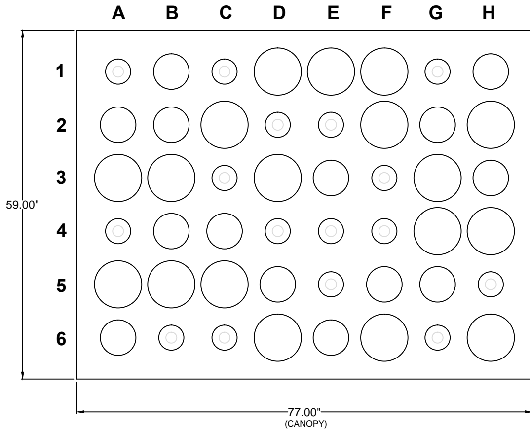
BOTTOM VIEW
