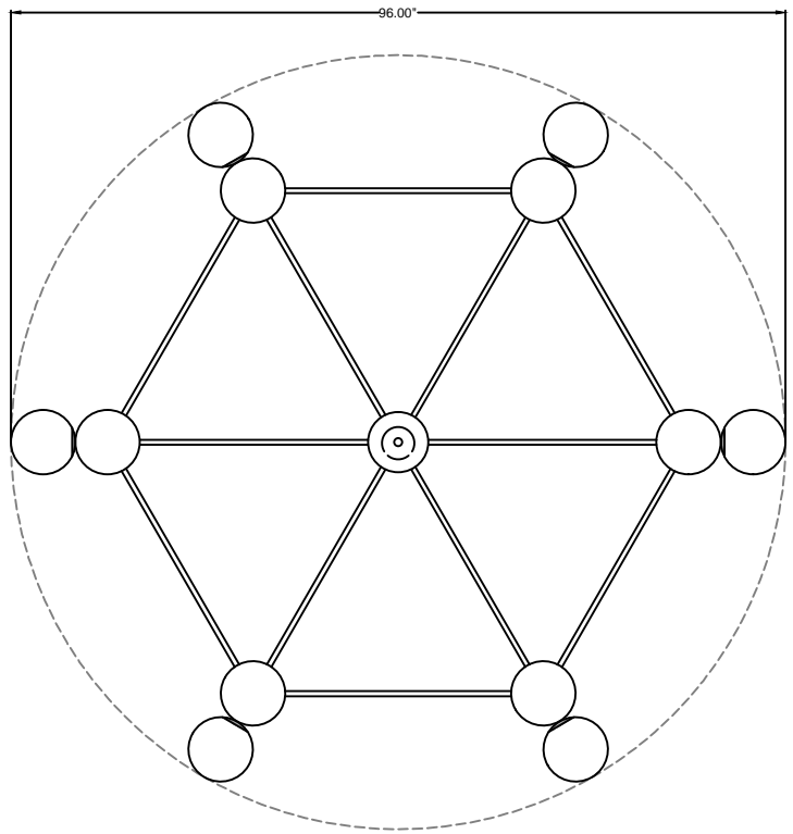
BOTTOM VIEW
